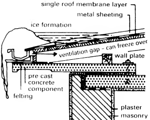
10 Cornice of pre-fabricated components; if the ventilation opening is too large a projection, it may freeze over
